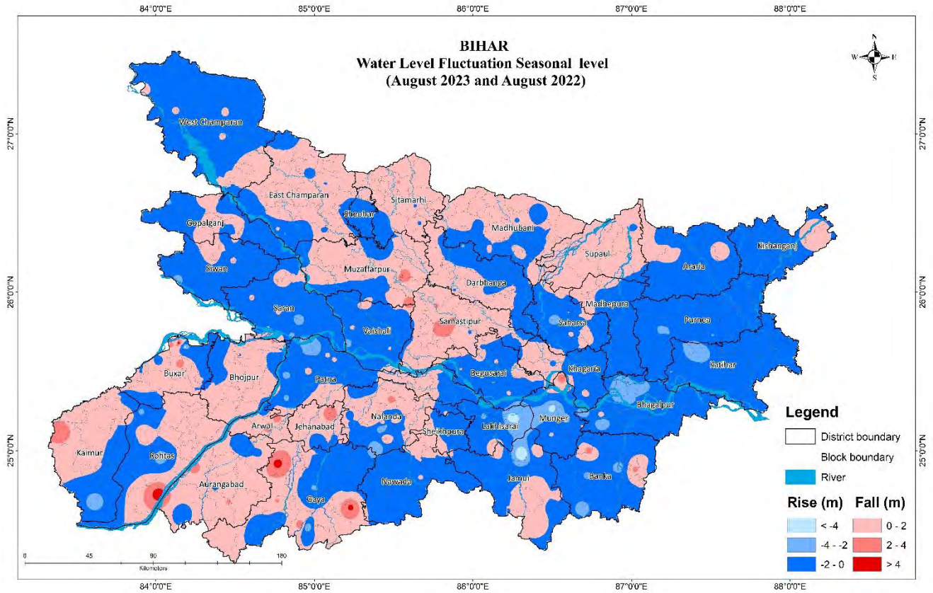
Figure 12: Fluctuation in ground water level between Aug. 2022 and Aug. 2023
