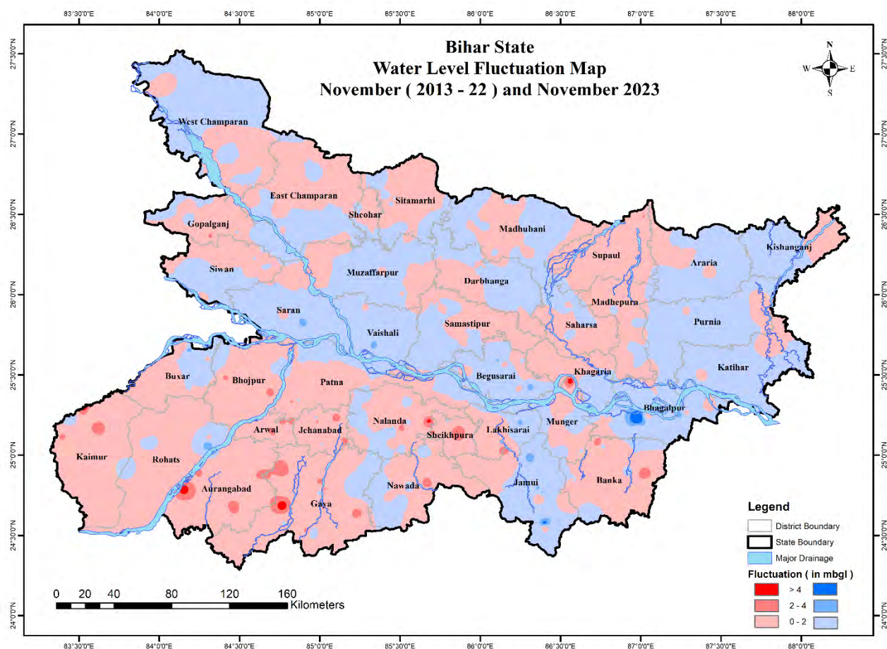
Figure 17: Fluctuation in water level between Nov. (mean) and Nov. 2023
