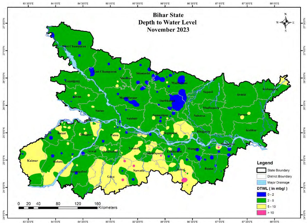
Figure 6: Depth to water level in November 2023
