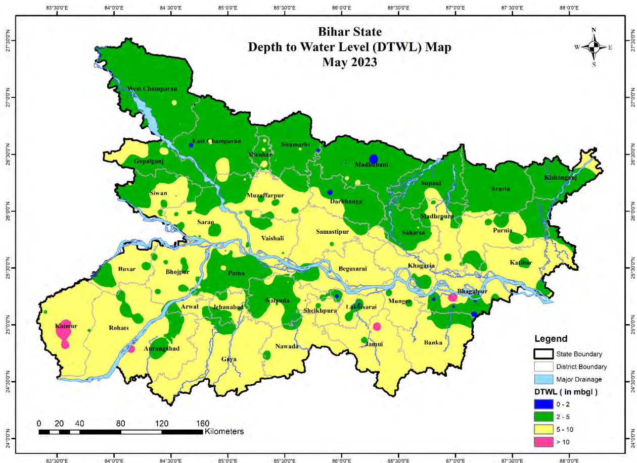
Figure 4: Depth to water level in May 2023
