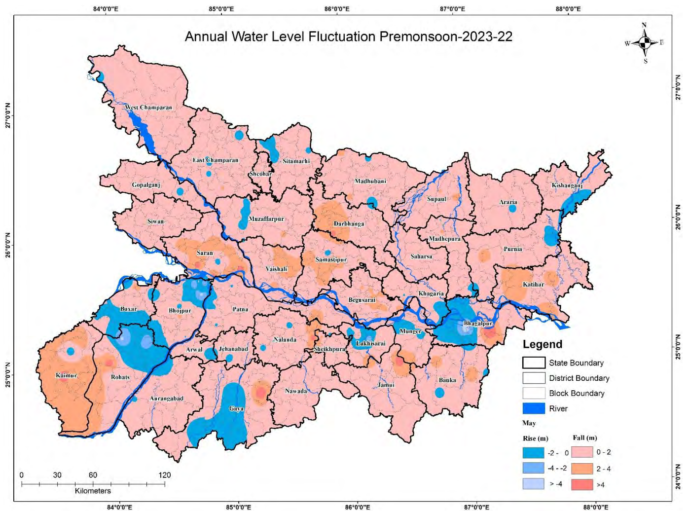
Figure 11: Fluctuation in ground water level between May 2022 and May 2023.
