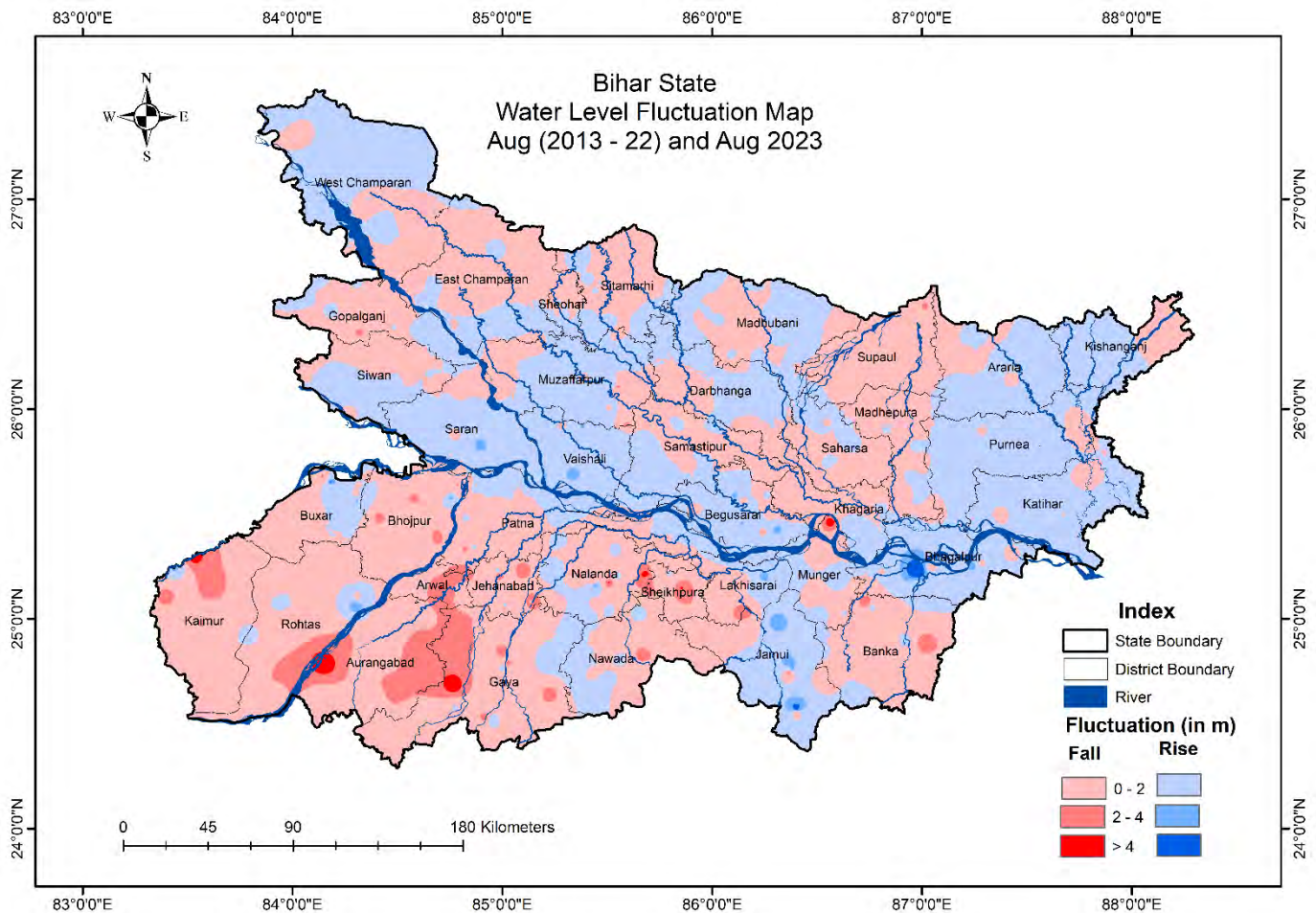
Figure 16: Fluctuation in water level between August (mean) and August 2023
