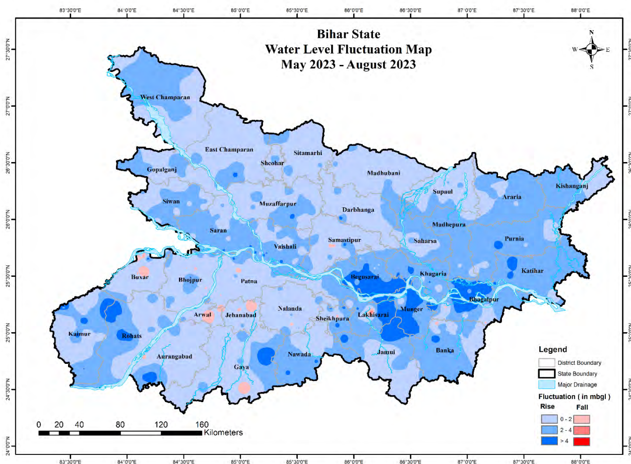
Figure 8: Water level Fluctuation between May 2023 and August 2023
