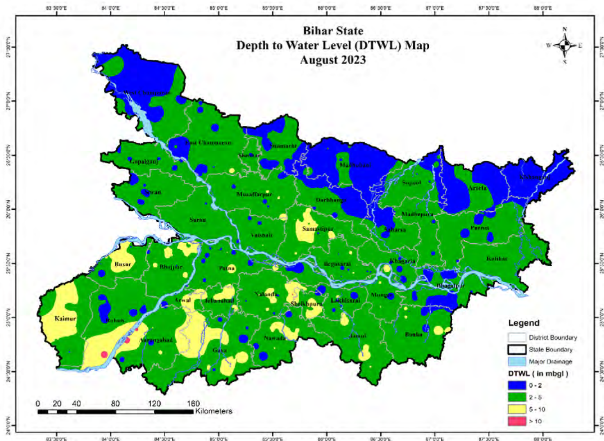
Figure 5: Depth to water level in August 2023
