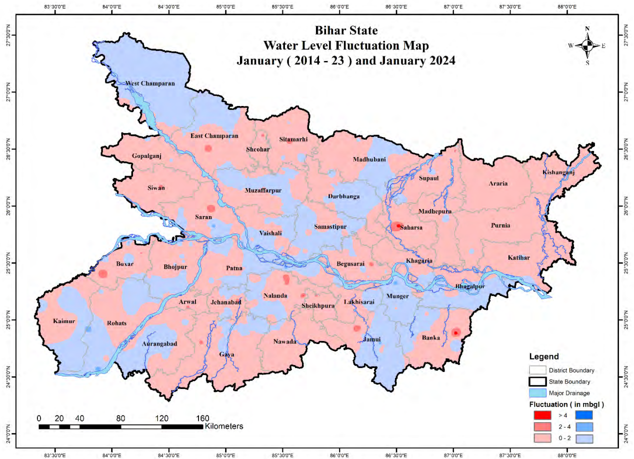
Figure 18: Fluctuation in water level Decadal Mean of January (2014-23) w.r.t January 2024
