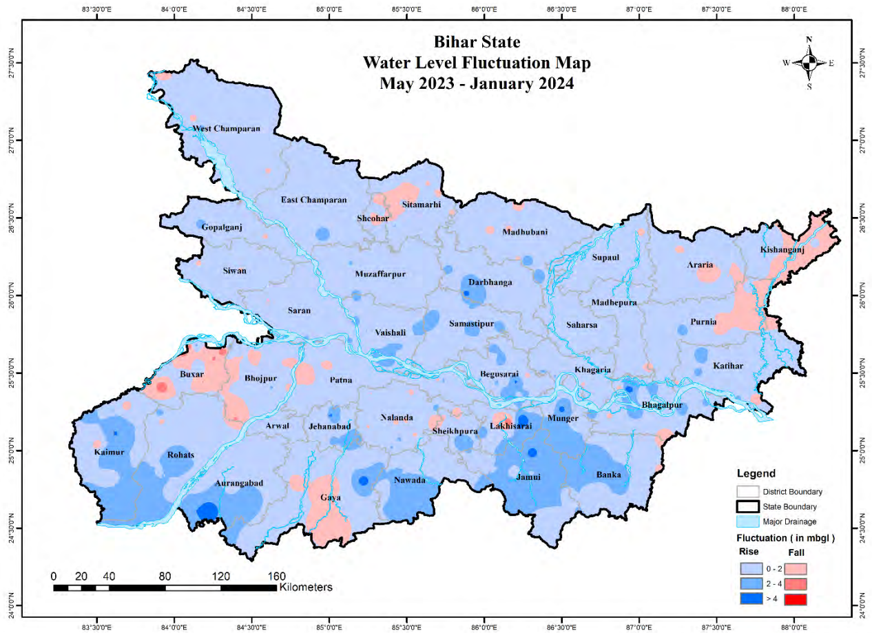
Figure 10: Fluctuation in ground water level between May 2023 and January 2024
