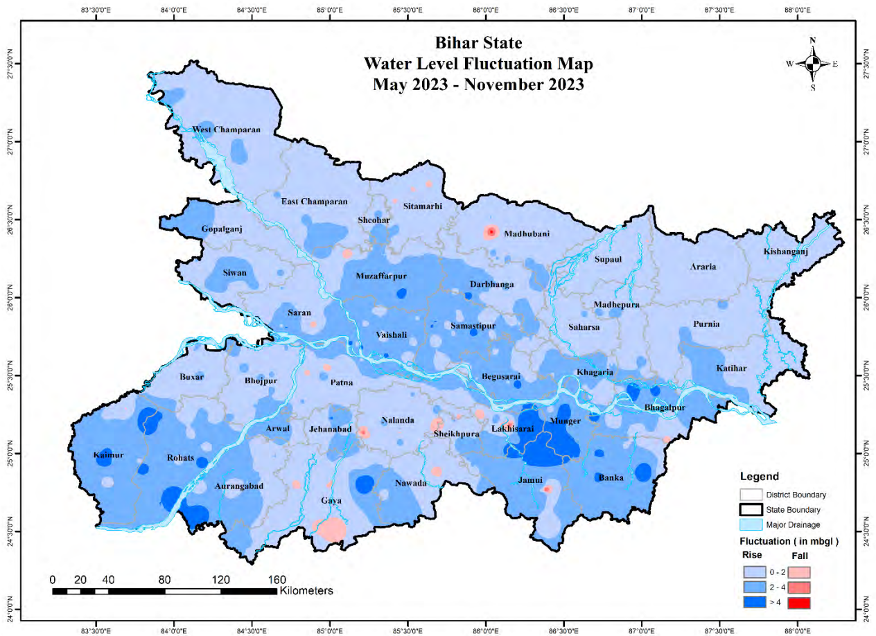
Figure 9: Fluctuation in ground water level between May 2023 and Nov. 2023
